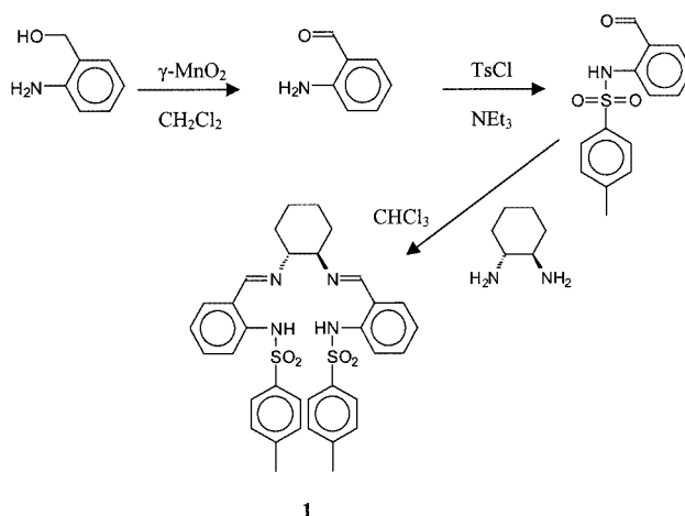
Scheme 2. Synthesis of 1 by Bermejo's method
