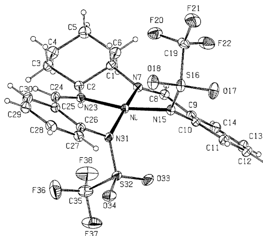
Figure 2. ORTEP view of complex 8
