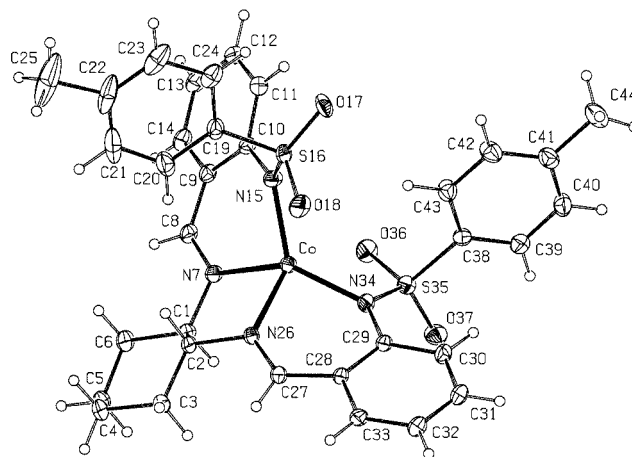
Figure 1. ORTEP view of complex 6
