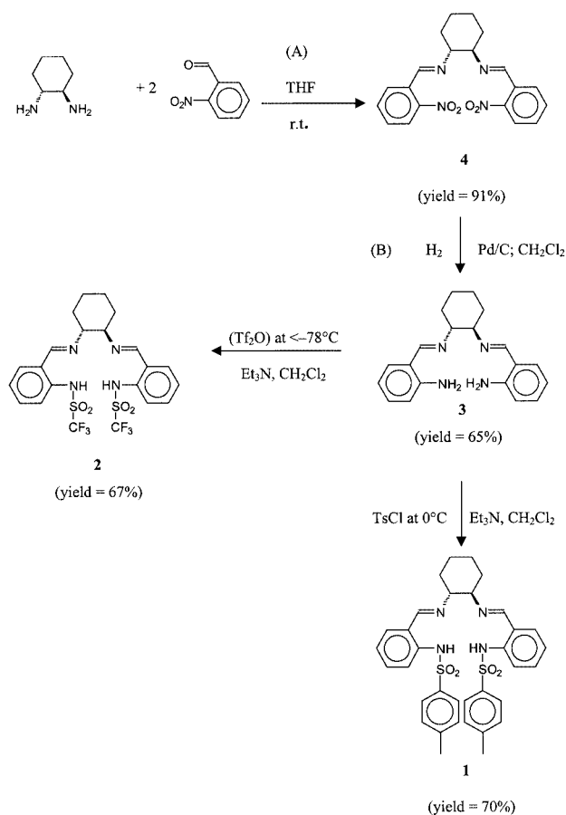
Scheme 1. General synthesis of N_4 Schiff bases 1–4
