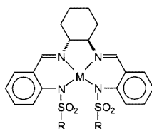
Scheme 4. General structural formula of complexes 5 , 6 , 7 and 8
